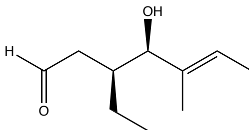
(3 S ,4 R , E )-3-ethyl-4-hydroxy-5-methyl-5-heptenal
